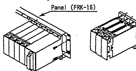
Fig.2 Wall Mounting
