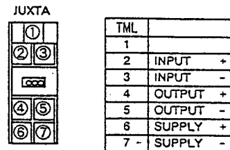
Fig.9 Wiring Diagram
