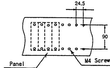
Fig.8 Terminal Arrangement
