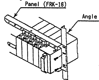
Fig.2 Wall Mounting
